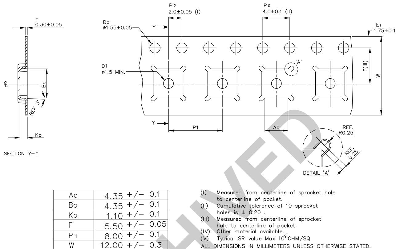
Figure 19. Tape dimensions
