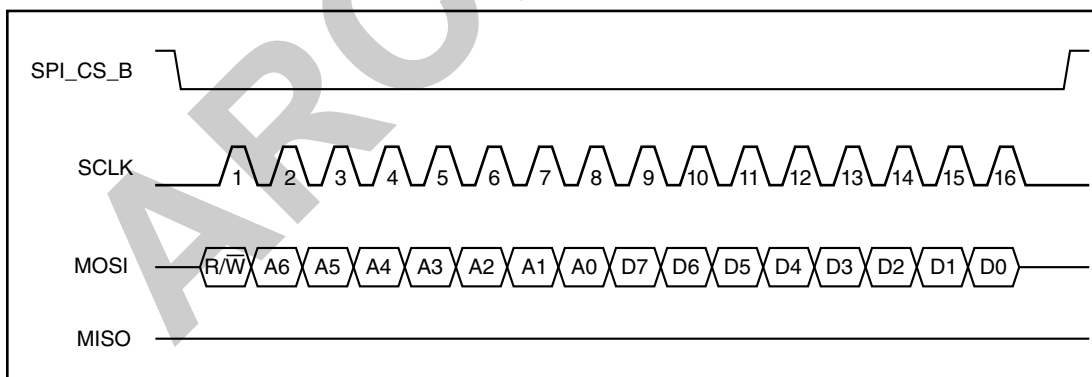
Figure 8. SPI single write operation. R/W = 1
