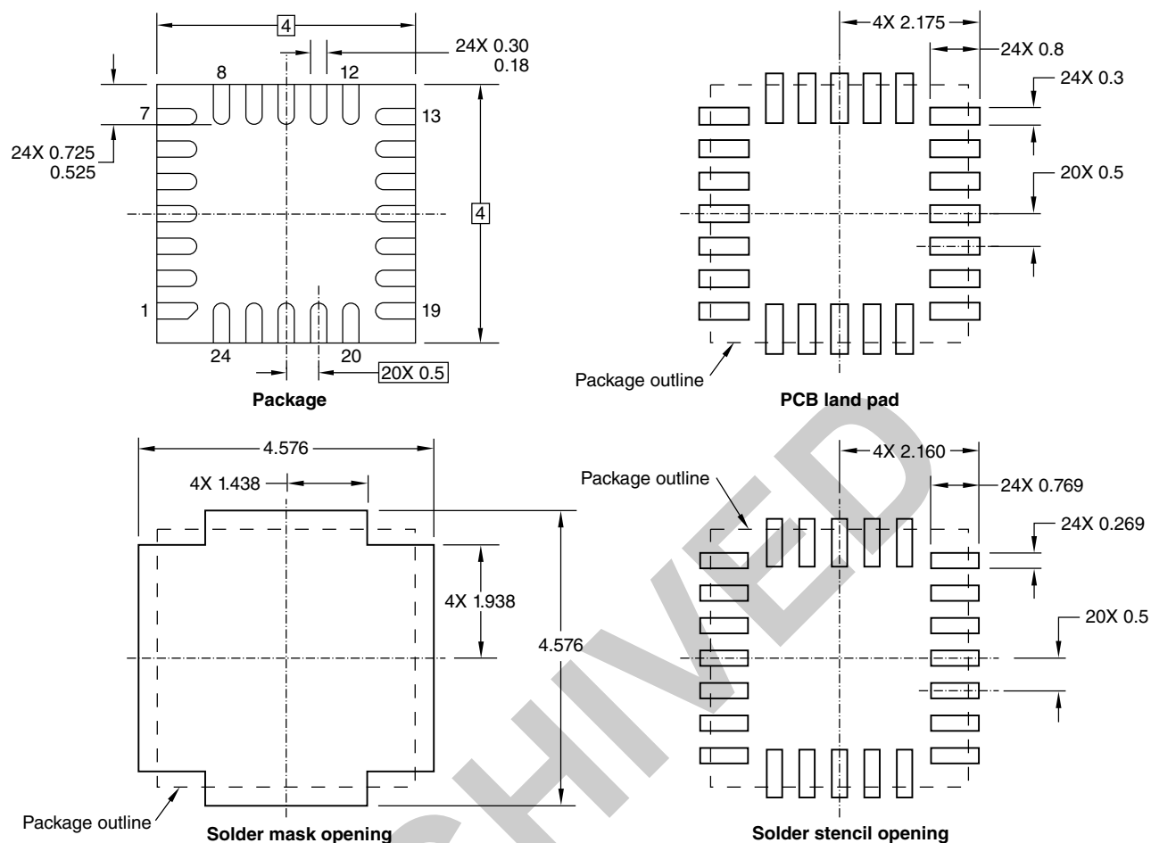
Figure 18. Footprint
