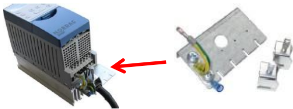
Figure 5: SK 500E with EMC kit SK EMC2-x
