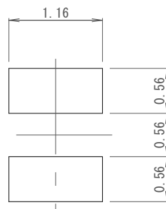
PCB Pattern
