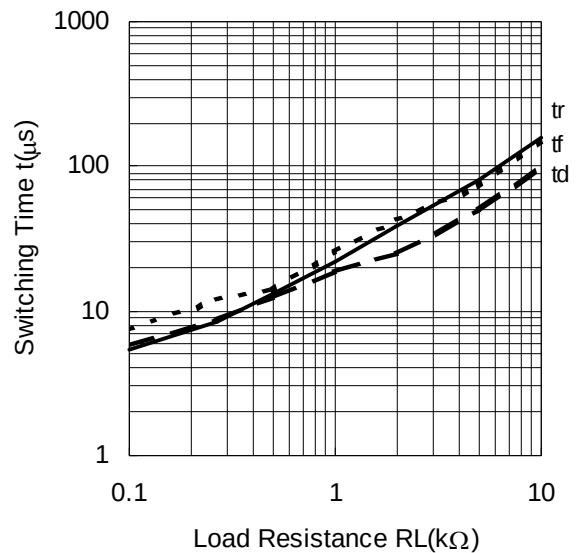
Switching Time vs. Load Resistance ( T_a=25^\circ\text{C} )
