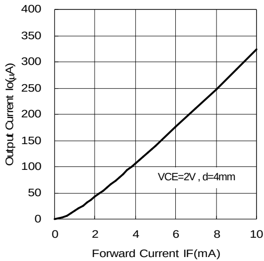
Output Current vs. Forward Current ( T_a=25^\circ\text{C} )
