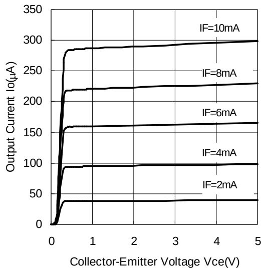
Output Characteristics ( T_a=25^\circ\text{C} )
