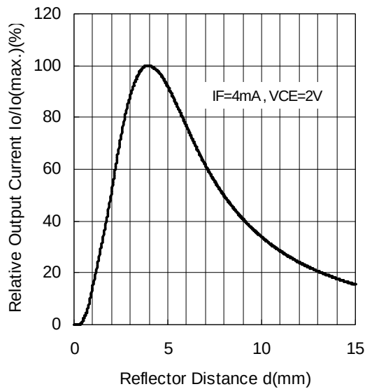
Output Characteristics ( T_a=25^\circ\text{C} )
