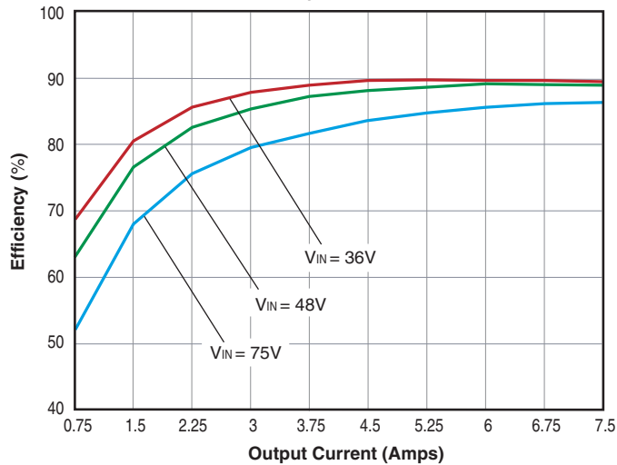
UHE-3.3/7500-D48 Efficiency vs. Load @ +25°C Ambient
