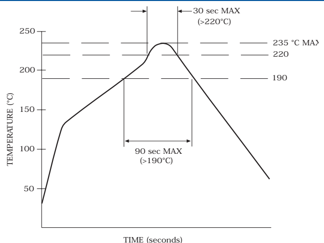
RECOMMENDED REFLOW PROFILE**
