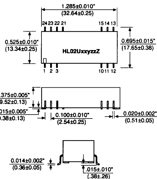
SMD PACKAGE
