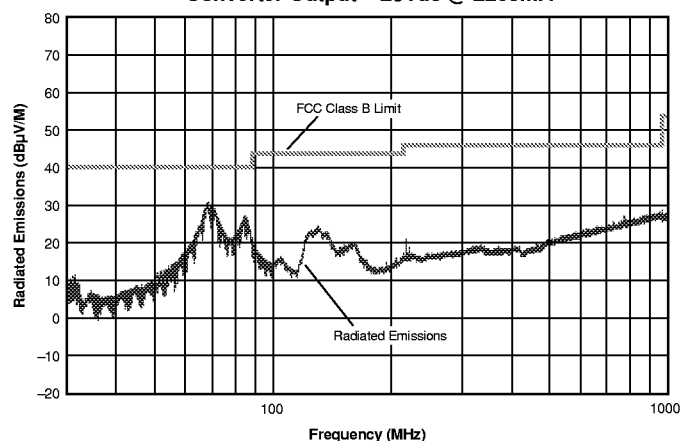
BWR-5/250-D12 Radiated Emissions FCC Part 15 Class B, 3 Meters Converter Output = \pm 5\text{Vdc} @ \pm 203\text{mA}
