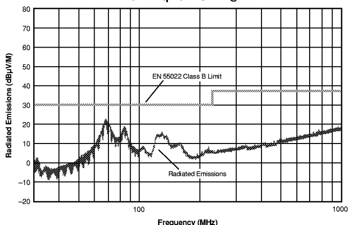
BWR-5/250-D12 Radiated Emissions EN 55022 Class B, 10 Meters Converter Output = \pm 5\text{Vdc} @ \pm 203\text{mA}
