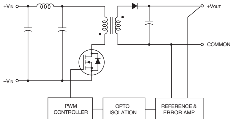
Figure 1. Simplified Schematic
