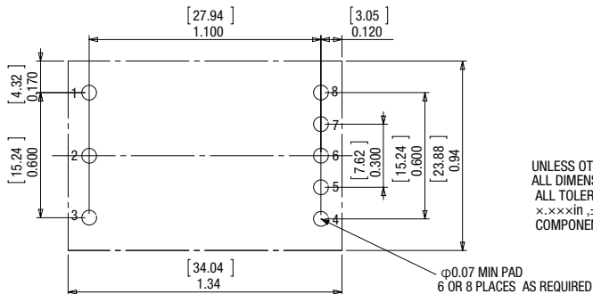
RECOMMEND PCB FOOTPRINT
