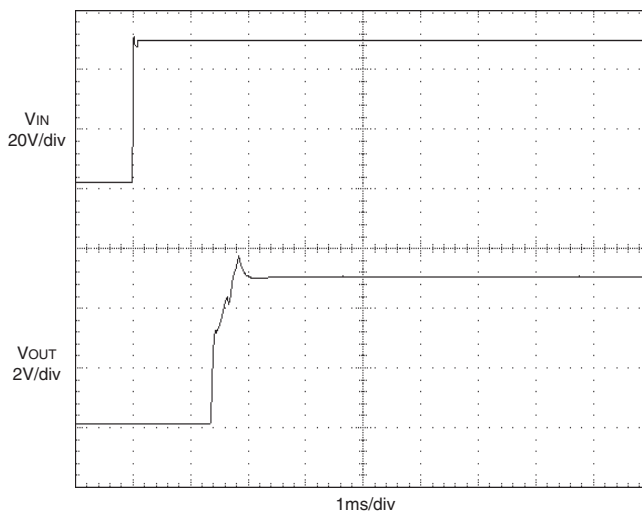
UWR-5/8-D48A Start-Up from V IN
