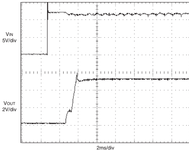
UWR-5/8-D24A Start-Up from V IN
