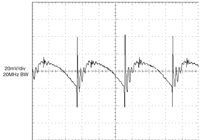
UWR-5/8-D24A Output Ripple and Noise (PARD)
