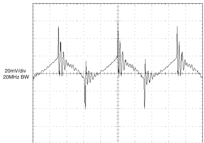
UWR-5/8-D48A Output Ripple and Noise (PARD)
