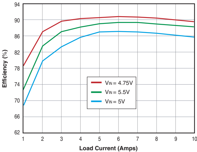
UNR-1.8/10-D5T/D5SM Efficiency vs. Line/Load
