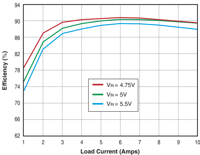
UNR-2.5/10-D5T/D5SM Efficiency vs. Line/Load
