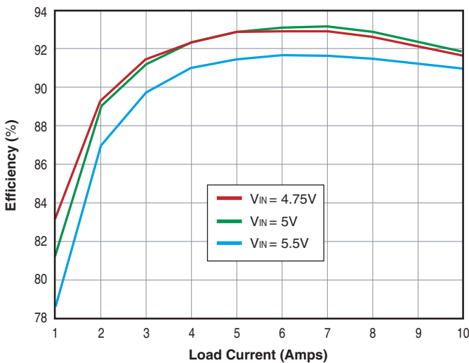
UNR-3.3/10-D5T/D5SM Efficiency vs. Line/Load
