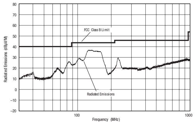
TWR-5/3000-15/500-D12A Radiated Emissions FCC Part 15 Class B, 3 Meters Converter Output = +5Vdc @ 2.7A and \pm 15Vdc @ \pm 450mA
