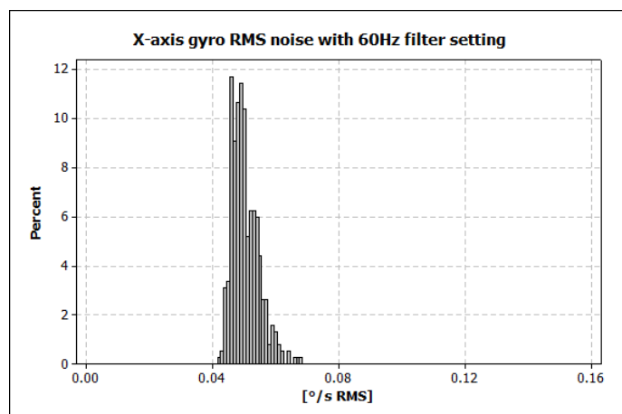
Figure 4. SCC2130-D08 gyro typical RMS noise in ^{\circ}/s_{RMS} .
