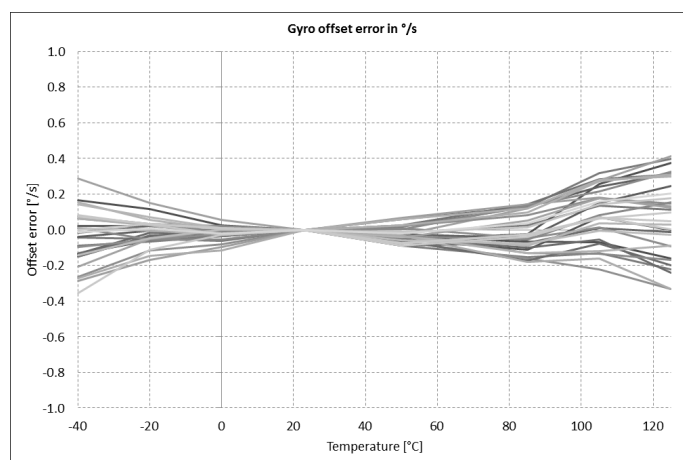
Figure 2. SCC2130-D08 gyro typical output temperature drift in ^{\circ}/s .
