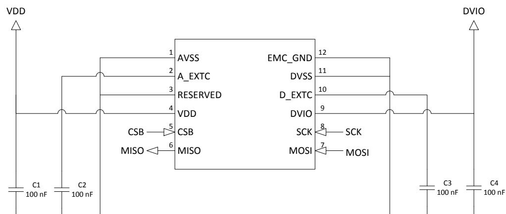
Figure 15 Application schematic
