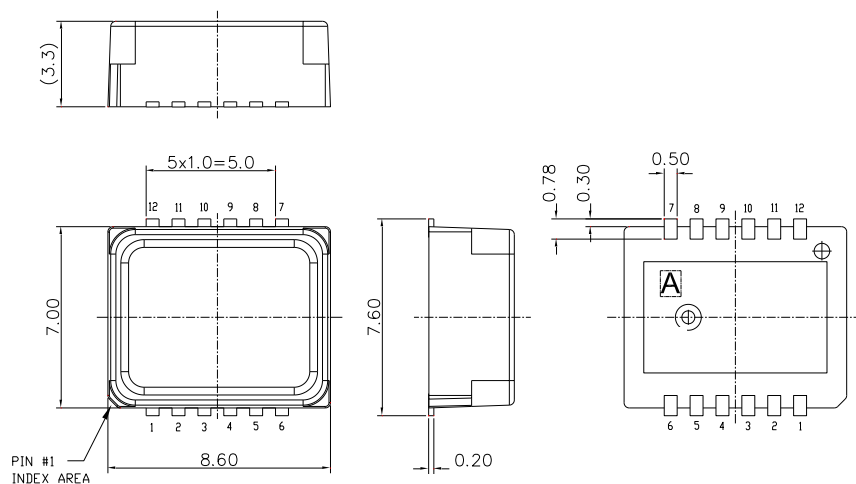
Figure 4. Housing dimensions
