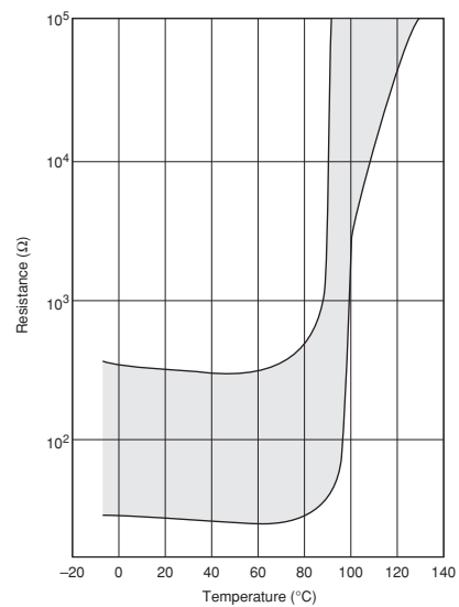
PTF_04BD222Q Type
