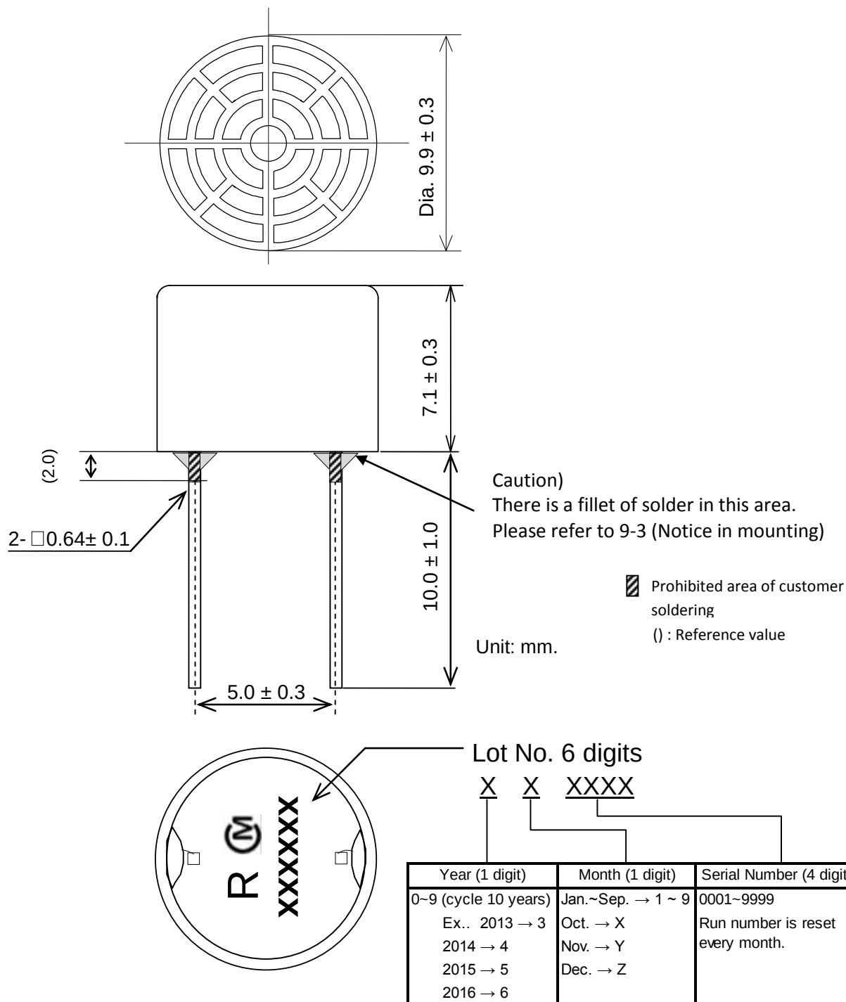
Fig.1: Product Dimension
