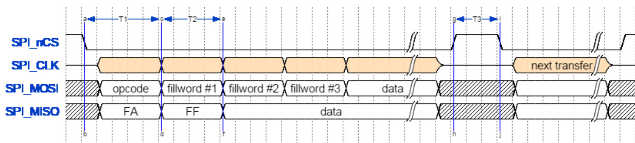
Figure 9: SPI timing
