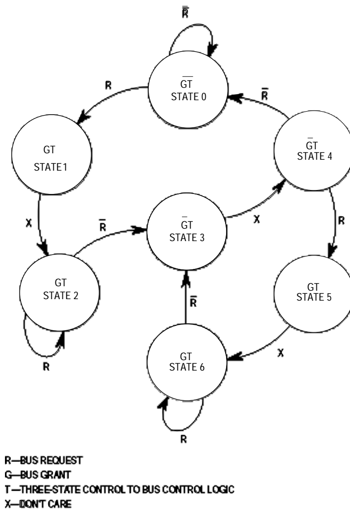
Figure 5-48. MC68EC020 Bus Arbitration State Diagram
