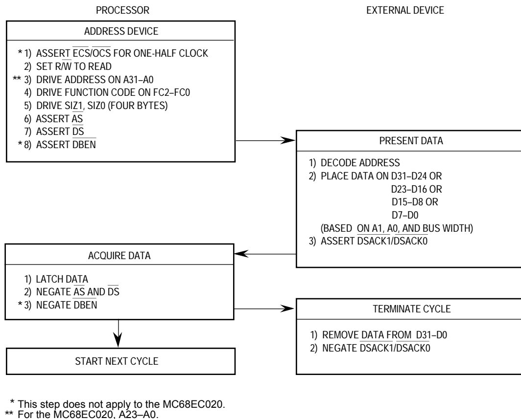
Figure 5-20. Byte Read Cycle Flowchart
