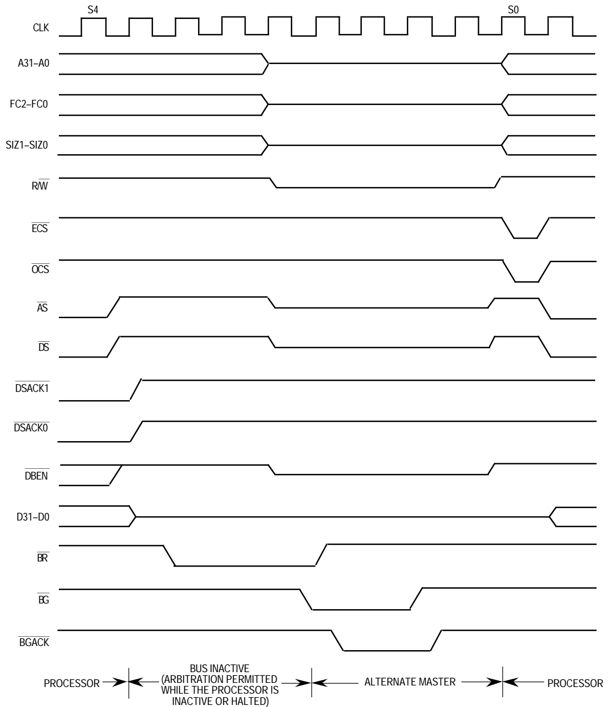
Figure 5-45. MC68020 Bus Arbitration Operation Timing—Bus Inactive
