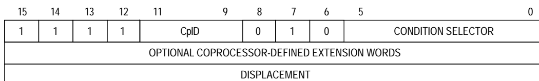
Figure 7-9. Branch on Coprocessor Condition Instruction Format (cpBcc.W)
