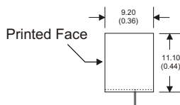
8 Pin SIL Package Non-Conductive Plastic
