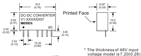
7 Pin SIL Package
