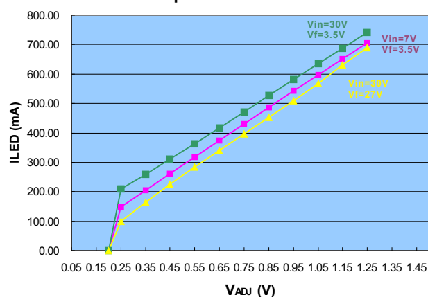
Output Current Vs VADJ
