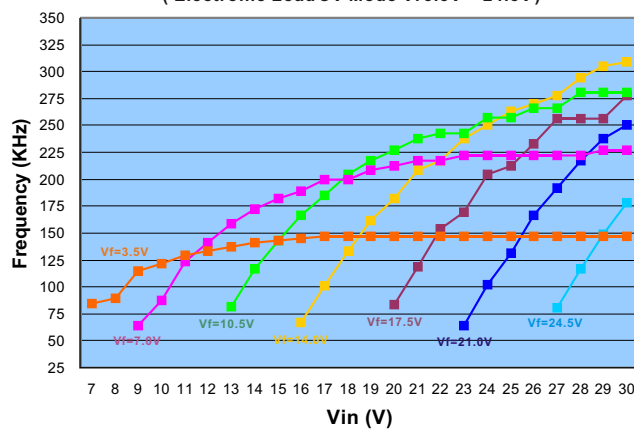
Operating Frequency vs Input Voltage (Electronic Load CV Mode Vf 3.5V ~ 24.5V)
