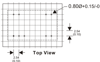
Recommended Footprint Details
