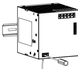
⑤Turn the Phillips screwdriver to the left to loosen the terminal screws, insert the head of the wire into the bottom of the terminal, and then turn the screwdriver to the right to tighten the terminal screws
