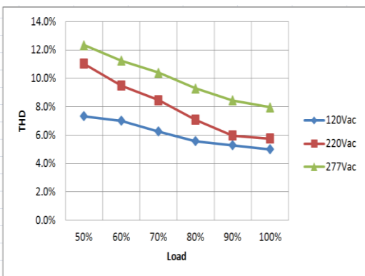
THD Curve(Ref.)
