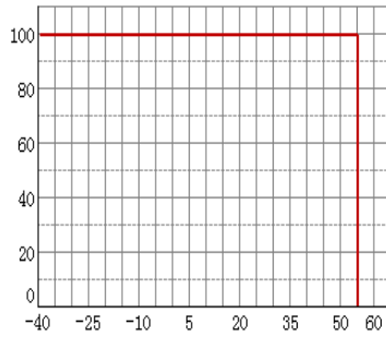
Derating Curve
