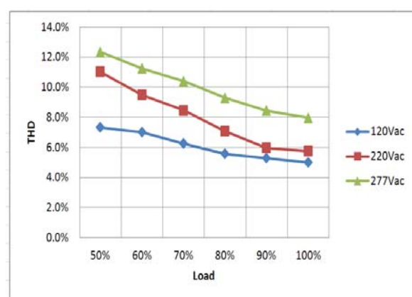
THD Curve
