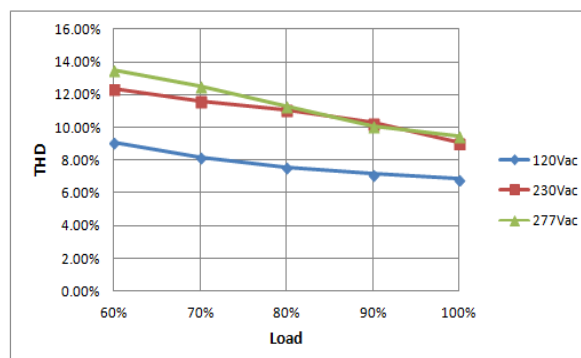
THD Curve
