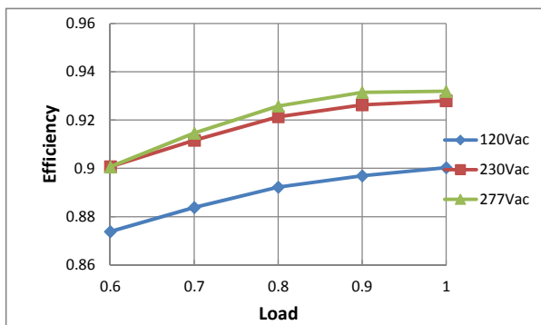
Efficiency VS. Load Curve (typ.)
