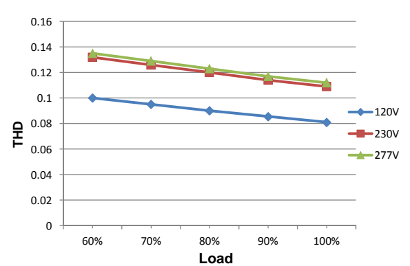
THD Curve
