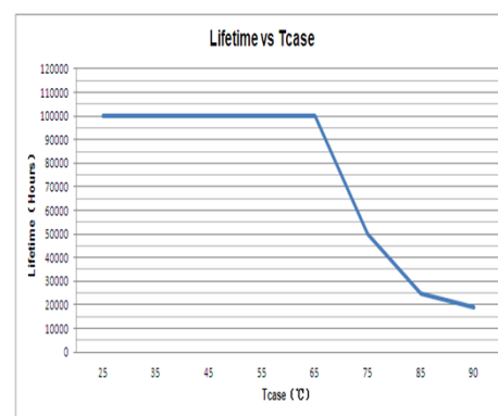
Life Time VS. Tcase Curve(Ref.Full load at 120Vac and 277Vac)
