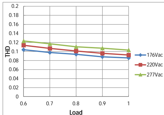
THD Curve
