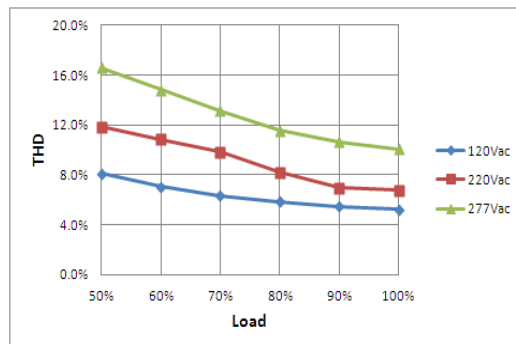
THD Curve
