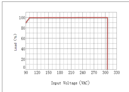
Derating Curve
