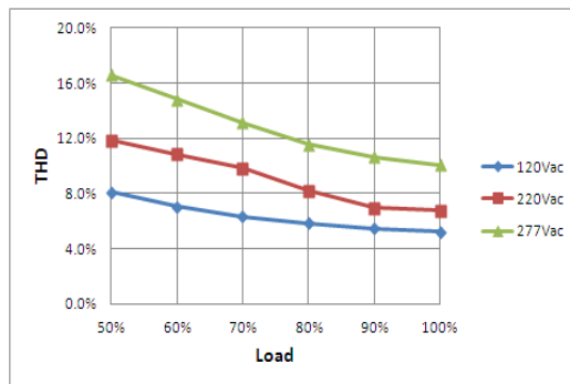
THD Curve
