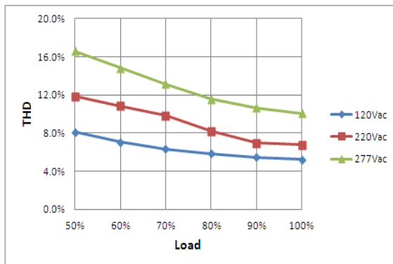
THD Curve
