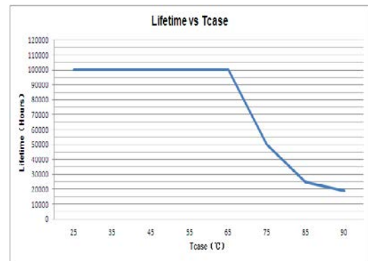
Life Time VS. Tcase (Ref.)
