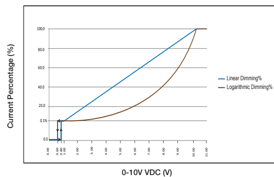
0-10V Curve
