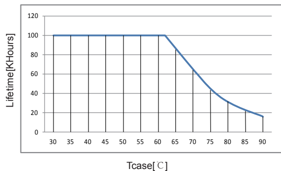
Lifetime VS.Tcase
