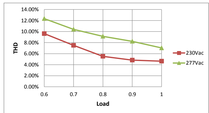
THD Curve
