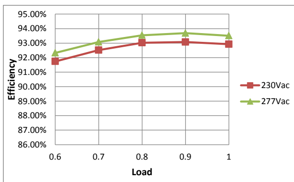
Efficiency VS. Load Curve (Io=4000mA)
