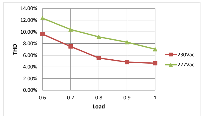
THD Curve
