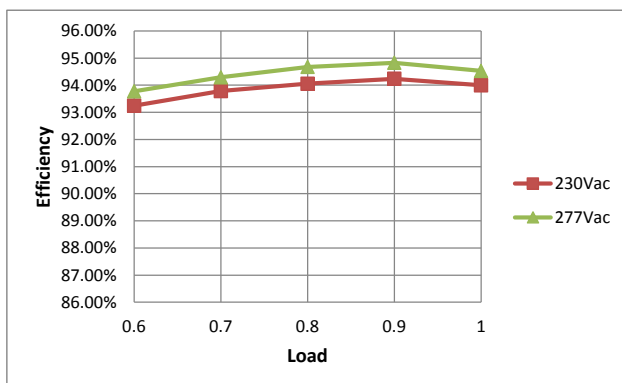
Efficiency VS. Load Curve (Io=700mA)
