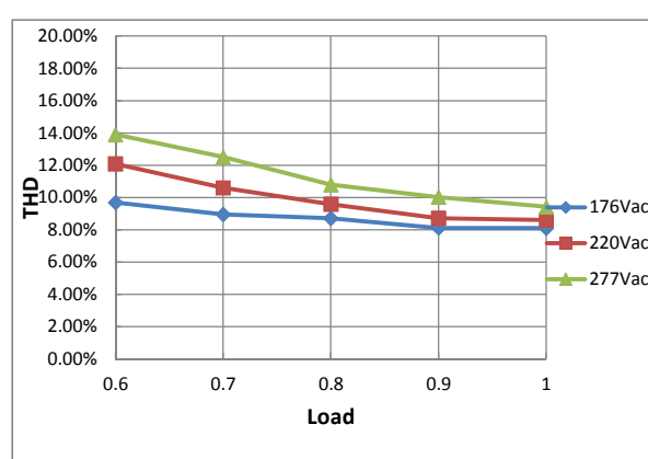
THD Curve
