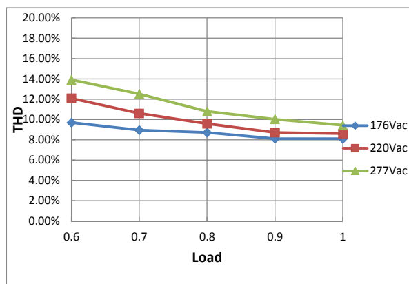
THD Curve
