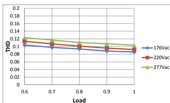
THD Curve
