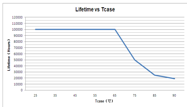
Lifetime VS. Tcase
