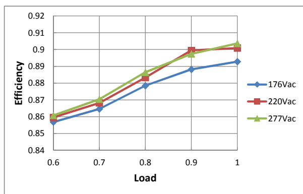
Efficiency VS. Load Curve(Model:700mA)
