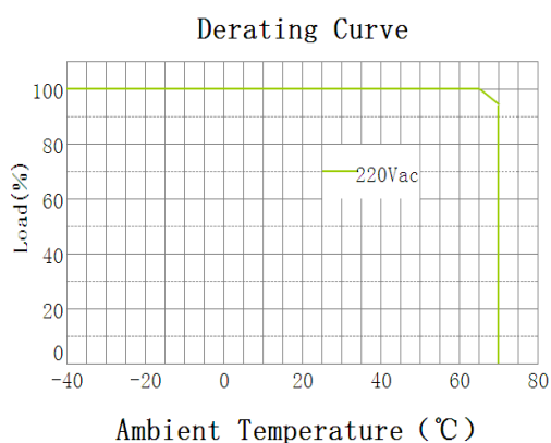
Derating Curve
