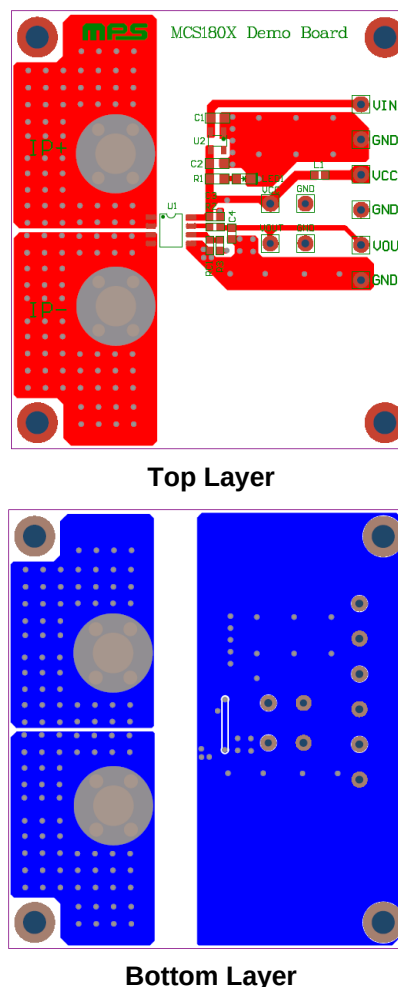
Figure 11: Recommended PCB Layout
