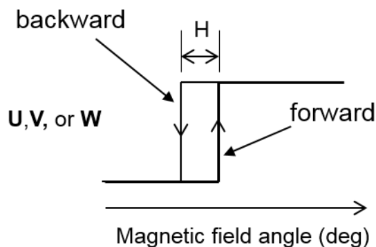
Figure 28: Hysteresis of the UVW Signal
