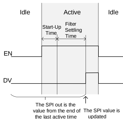
Figure 30: Signal Timing for External Control
