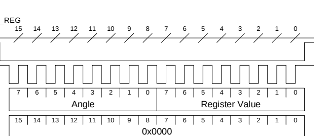
Figure 16: Overview of a Write Register Operation with Two 16-Bit Frames
