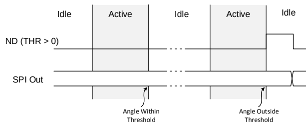
Figure 39: Using the ND Pin as a WOC Signal with a Non-Zero Threshold Setting.
