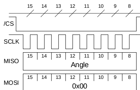
Figure 11: Partial 8-Bit SPI Angle Reading Diagram
