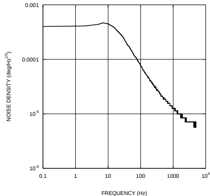
Noise Spectrum at 50mT and \tau = 16\text{ ms}
