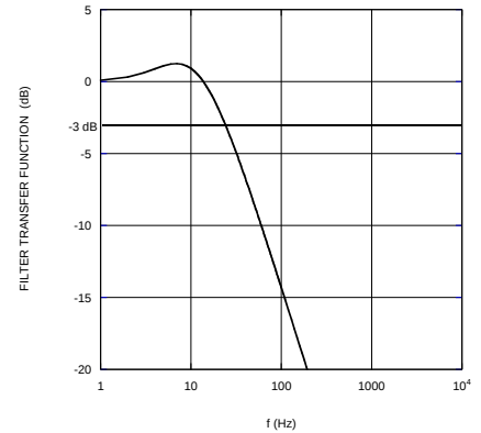
Filter Transfer Function at \tau = 16\text{ ms}
