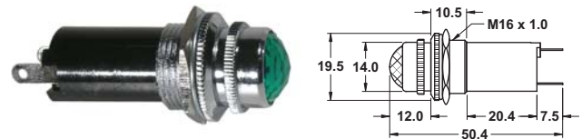
T 3-1/4 (10mm) screw base
