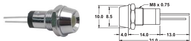
Chrome plated LED indicator
