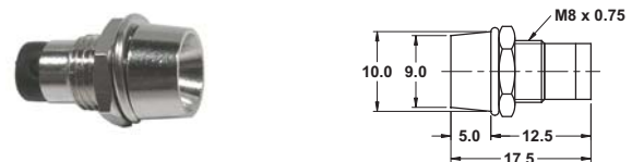
Chrome plated LED holder
