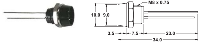
Black plastic bezel LED indicator
