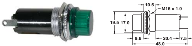
T 3-1/4 (10mm) bayonet base
