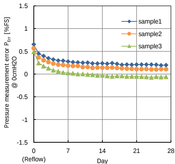
Fig. 23.8 Pressure measurement error P_{Err} @0cmH 2 O Reflow drift
