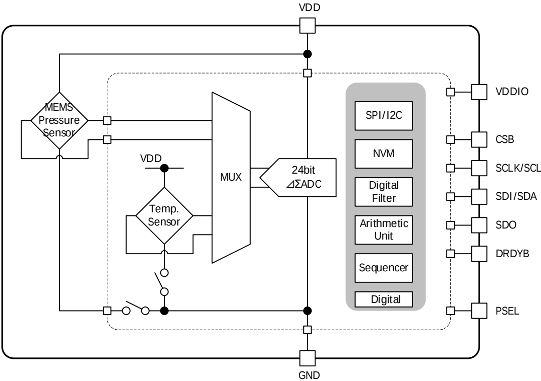
Fig. 1 Block diagram
