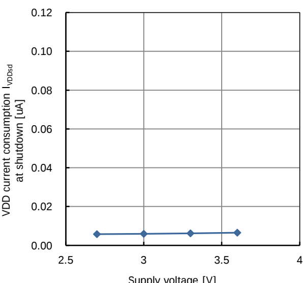
Fig. 22.4 VDD current consumption I_{VDDsd} at shutdown supply voltage characteristic
