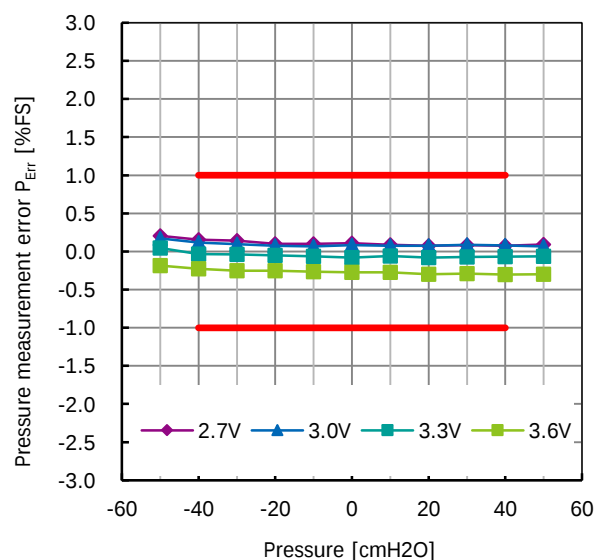
Fig. 23.5 Pressure measurement error P_{Err} supply voltage characteristic
