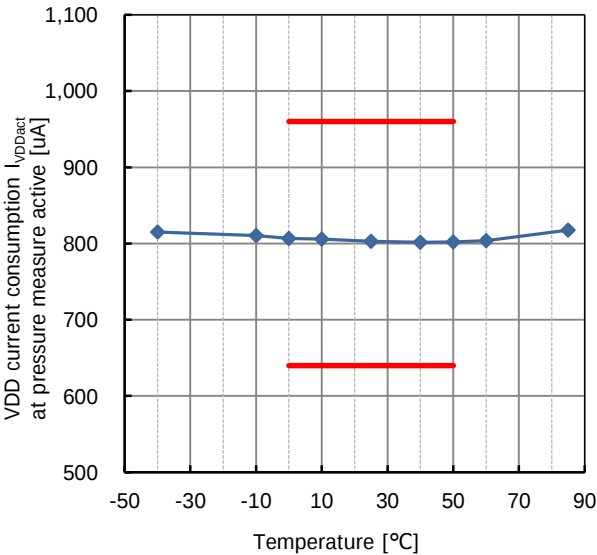
Fig. 22.1 VDD current consumption I_{VDDact} at pressure measure active temperature characteristic
