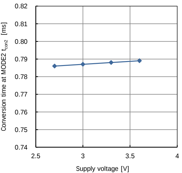
Fig. 22.12 Conversion time at MODE 2 supply voltage characteristic
