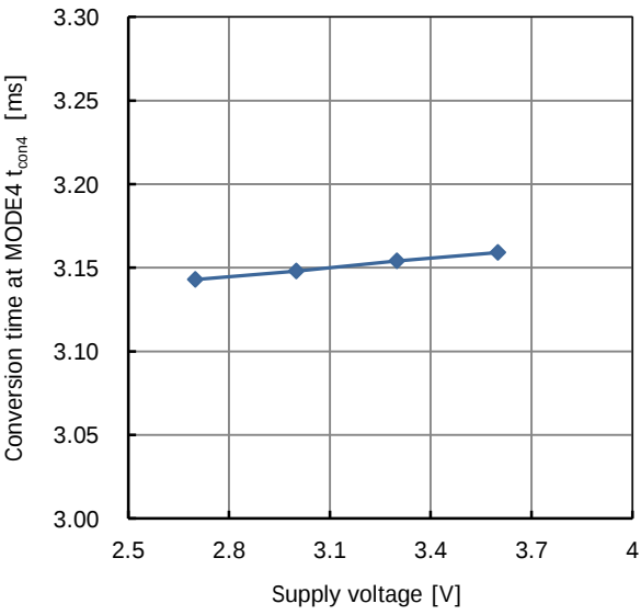
Fig. 22.16 Conversion time at MODE 4 supply voltage characteristic
