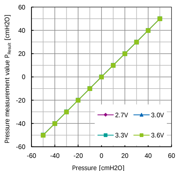
Fig. 23.2 Pressure measurement value P_{\text{Result}} supply voltage characteristic
