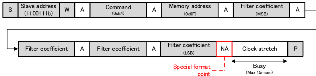
Fig. 19 I2C MACRAM Write format
