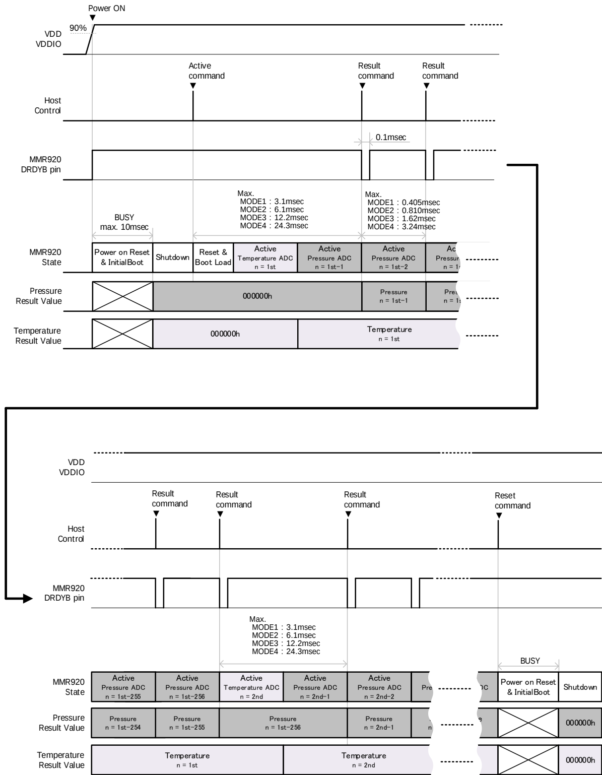
Fig. 8 Timing Chart
