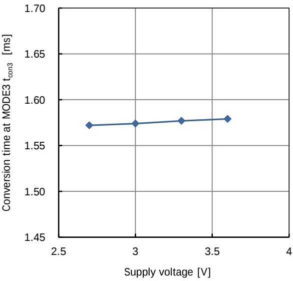
Fig. 22.14 Conversion time at MODE 3 supply voltage characteristic
