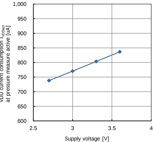
Fig. 22.3 VDD current consumption I_{VDDsd} at shutdown temperature characteristic
