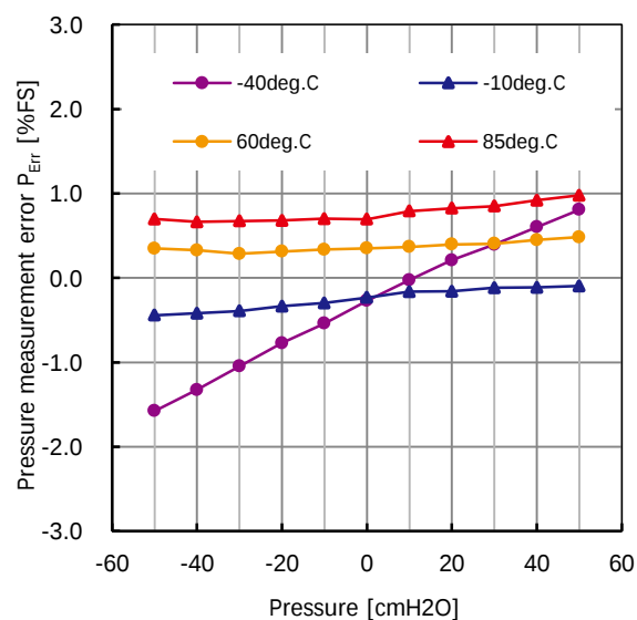
Fig. 23.4 Pressure measurement error P_{\text{Err}} temperature characteristic -40~85deg.C
