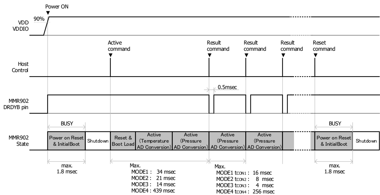
Fig. 17 Timing Chart
