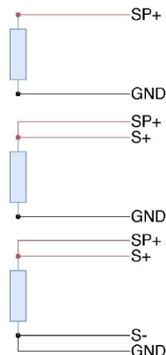
Resistance Thermometer
