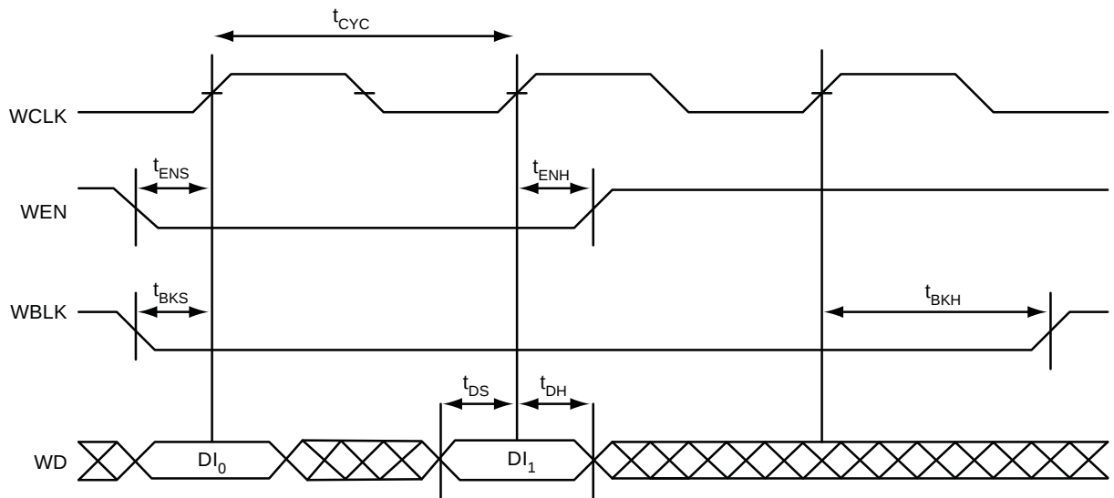
Figure 2-50 • FIFO Write
