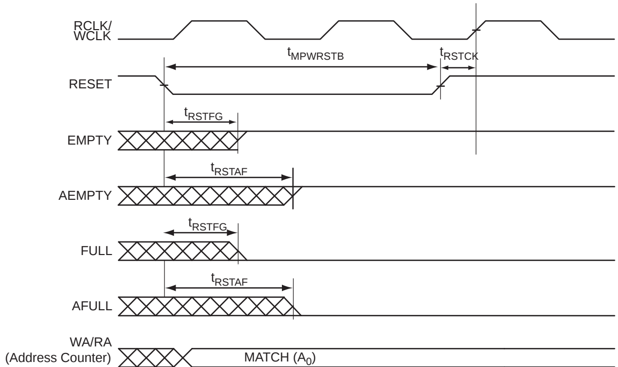
Figure 2-51 • FIFO Reset
