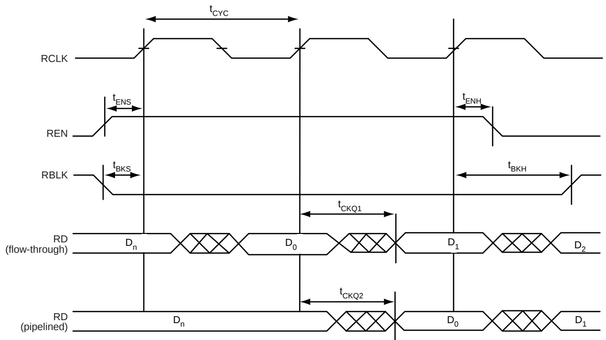
Figure 2-49 • FIFO Read
