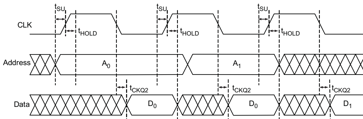
Figure 2-56 • Timing Diagram
